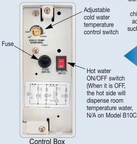
Control Box
